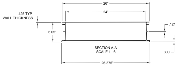
24" x 6" Riser Cutaway
